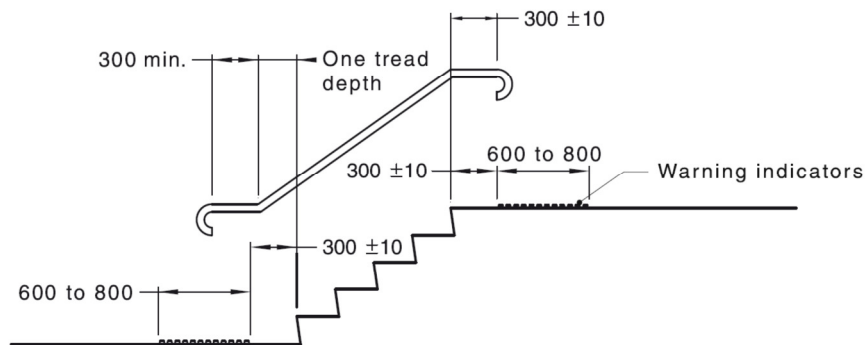
Figure 8: Handrail Details
